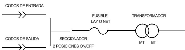
DIAGRAMA UNIFILAR PEDESTAL ANILLO (MALLA)
