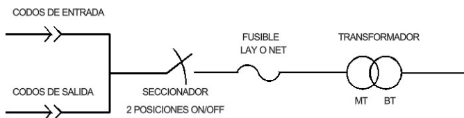
DIAGRAMA UNIFILAR PEDESTAL RADIAL
